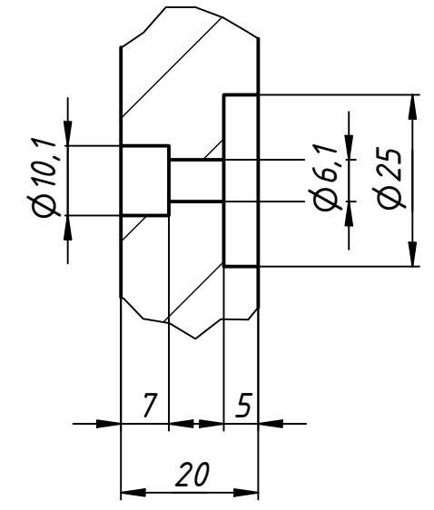
B (1:1)
